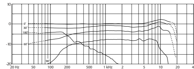
Typical on- and off-axis frequency response of 4099 at 20 cm (7.9 in) distance
