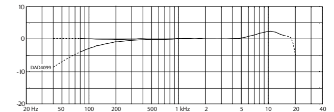
Typical frequency response of 4099 with DAD4099 XLR adapter at 20 cm (7.9 in) distance
