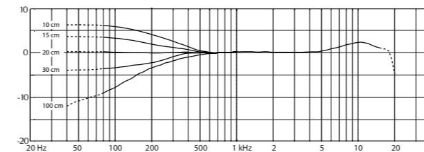
The proximity effect exhibited by 4099
