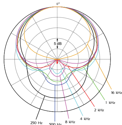
Typical characteristics of 4099 (normalized)
