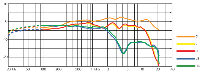
Typical frequency response of DPA 5100 at 0 degrees
