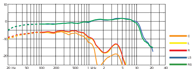
Typical frequency response of DPA 5100 at 180 degrees
