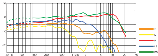
Typical frequency response of DPA 5100 at 90 degrees
