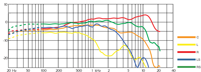
Typical frequency response of DPA 5100 at 60 degrees
